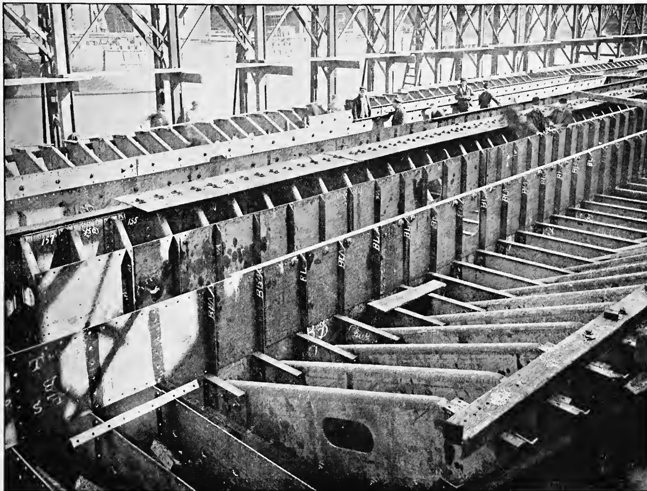
STUART'S CHANNEL SYSTEM OF CONSTRUCTION.—Showing keel, keelsons, intercostals and floors.
